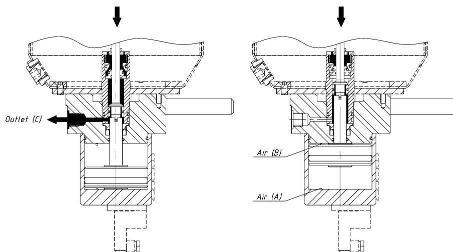
Fig.1: Illustration of operating principle
